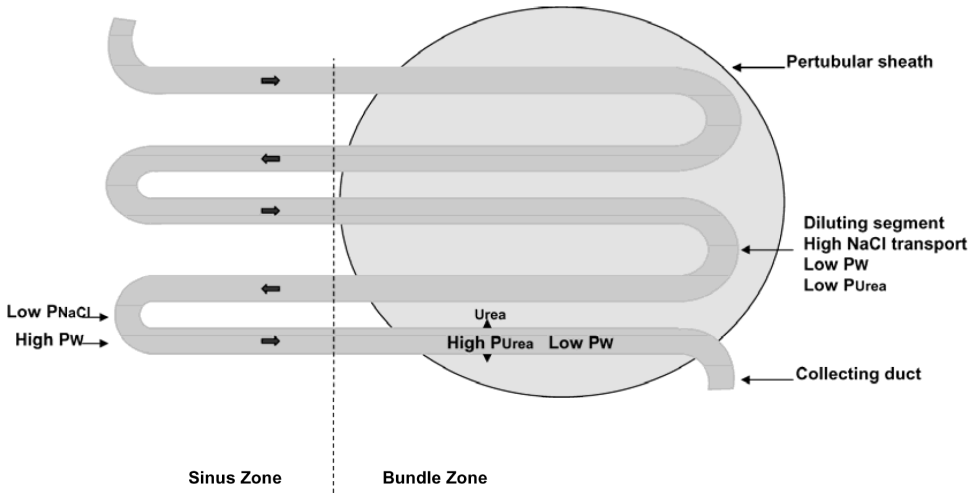
Figure 2. Hypothesised model of passive renal urea reabsorption in S. acanthias based on the presence of the countercurrent arrangement of nephron segments in the kidney bundle zone. The countercurrent arrangement is composed of four nephron segments grouped to form two loops and together with a fifth segment are enclosed by a continuous peritubular sheath. The diluting nephron segment in the dorsal bundle of the peritubular sheath has a high rate of active salt absorption and low water and urea permeability, while the segment in the sinus zone has low salt and high water permeability. The distal tubule has high urea and low water permeability, permitting diffusion of urea from the tubular fluid into intrabundle space (small black arrow heads). Small black broad arrows indicate direction of axial tubular fluid flow. Water, salt and urea permeability designated as P_W , P_{NaCl} and P_{Urea} , respectively. Figure re-drawn and used with permission from Friedman and Hebert 1990.
