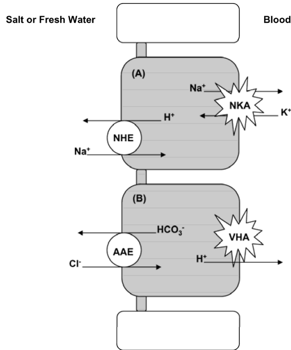
Figure 3. Hypothesised model of acid–base and NaCl transport in the elasmobranch gill. A distinct mitochondria-rich cell (A) with \text{Na}^+ , \text{K}^+ -ATPase is likely the site of hydrogen ion excretion in an electroneutral exchange for environmental sodium. Basolateral \text{Na}^+ , \text{K}^+ -ATPase (NKA) actively pumps gill intracellular sodium ions across the basolateral membrane into the plasma, maintaining low intracellular sodium concentrations, favourable for apical sodium uptake in exchange for hydrogen excretion via a sodium/hydrogen exchange (NHE) mechanism. Another distinct mitochondrion rich cell (B) with V- \text{H}^+ -ATPase is likely the site of chloride ion uptake and bicarbonate ion excretion. Basolateral V- \text{H}^+ -ATPase (VHA) seems to actively pump hydrogen ions across the basolateral membrane, creating an intracellular bicarbonate concentration, favourable for apical bicarbonate secretion and chloride ion uptake via an apical anion exchanger (AAE). Figure re-drawn and used with permission from Piermarini and Evans, 2001 and The Company of Biologists Ltd.
