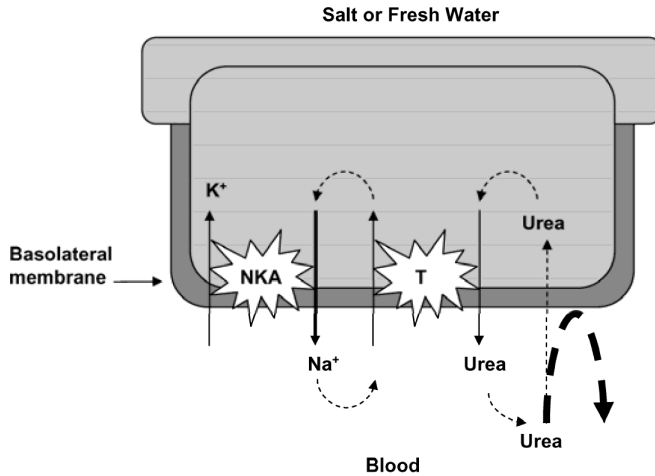
Figure 1. Hypothesised model of urea retention and transport at the elasmobranch gill. Basolateral gill membrane of S. acanthias minimises entry of urea (thick dashed arrow) due to a high cholesterol-to-phospholipid ratio. Intracellular urea that leaks back into the gills is transported across the basolateral membrane via a \text{Na}^+ : Urea antiporter (T), energised by the continual removal of \text{Na}^+ from the gill via basolateral \text{Na}^+ , \text{K}^+ -ATPases (NKA). Figure re-drawn and used with permission from Evans et al. 2005.
